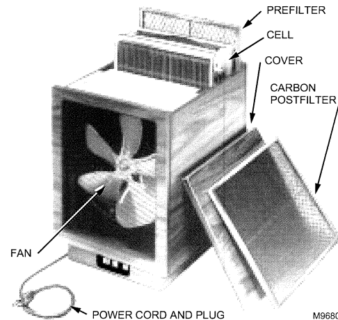
Fig. 1—F59A components.
