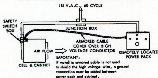
WIRING FOR REMOTE POWER PACK
