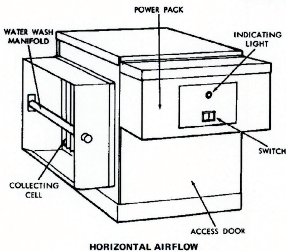
HORIZONTAL AIRFLOW
