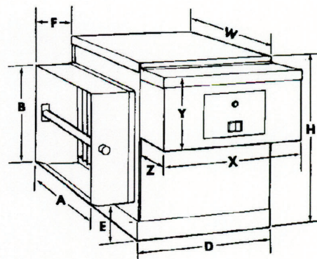
HORIZONTAL AIRFLOW UNITS MODEL WW-14-H MODEL WW-20-H
