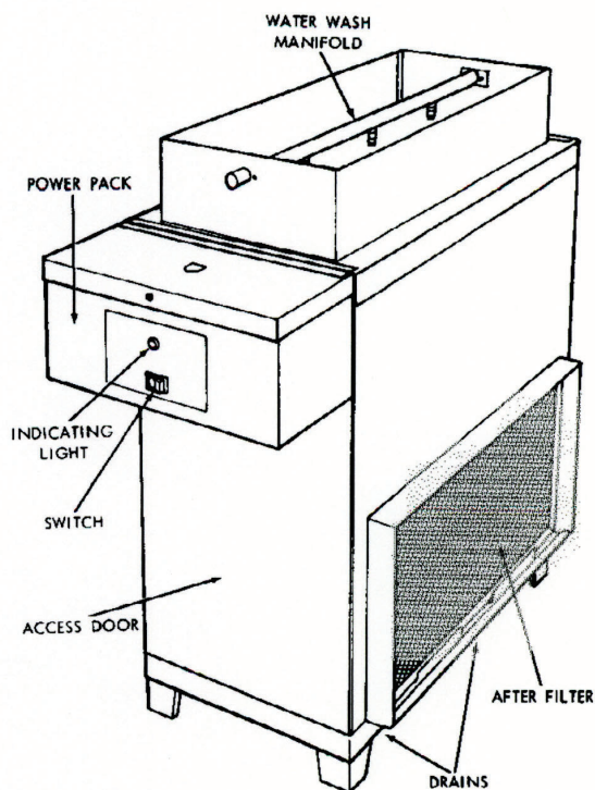
VERTICAL (DOWN) AIRFLOW
